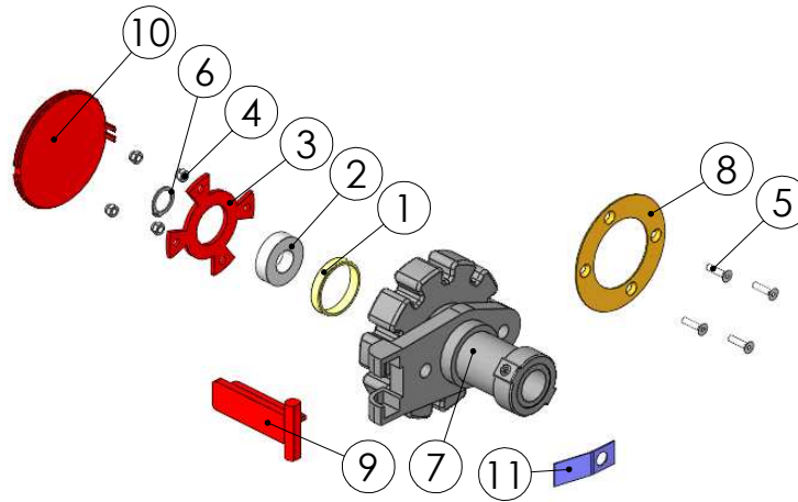
Hand wheel 98837403
