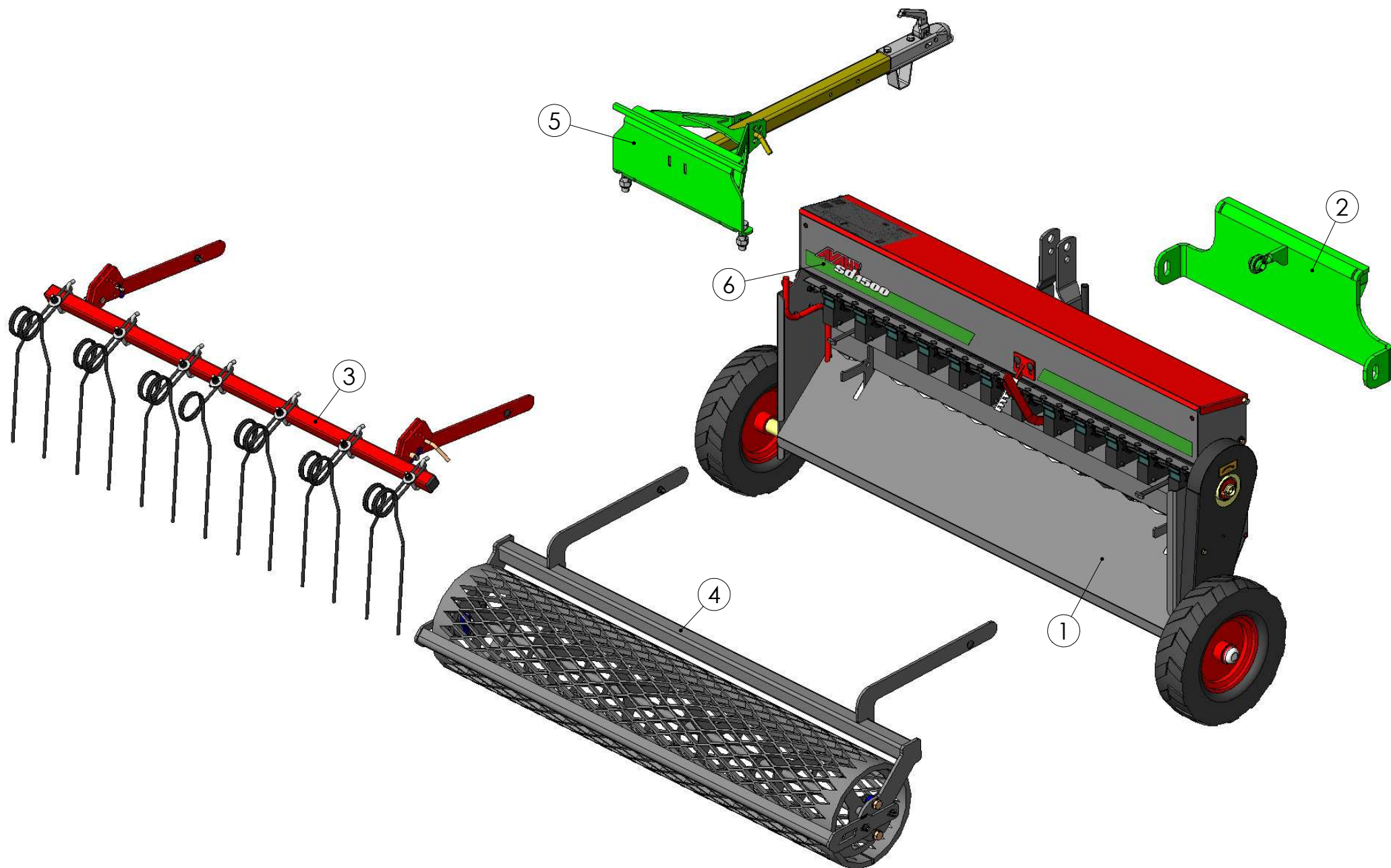
99480702 AVANT sd1500 + mounting adapter (Avant code: A449473)
