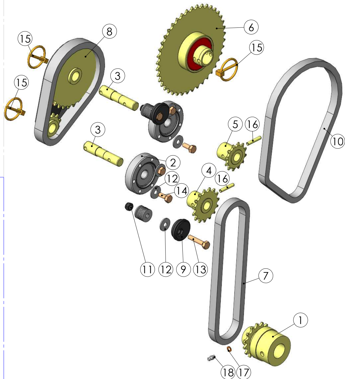
99486203 Transmission
